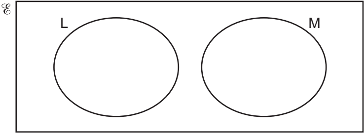
Venn diagram 2:
