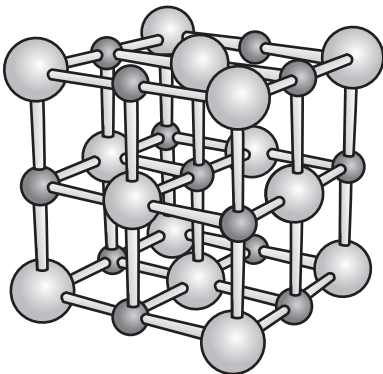
Ball-and-stick model
