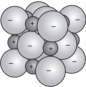
Space-filling model
